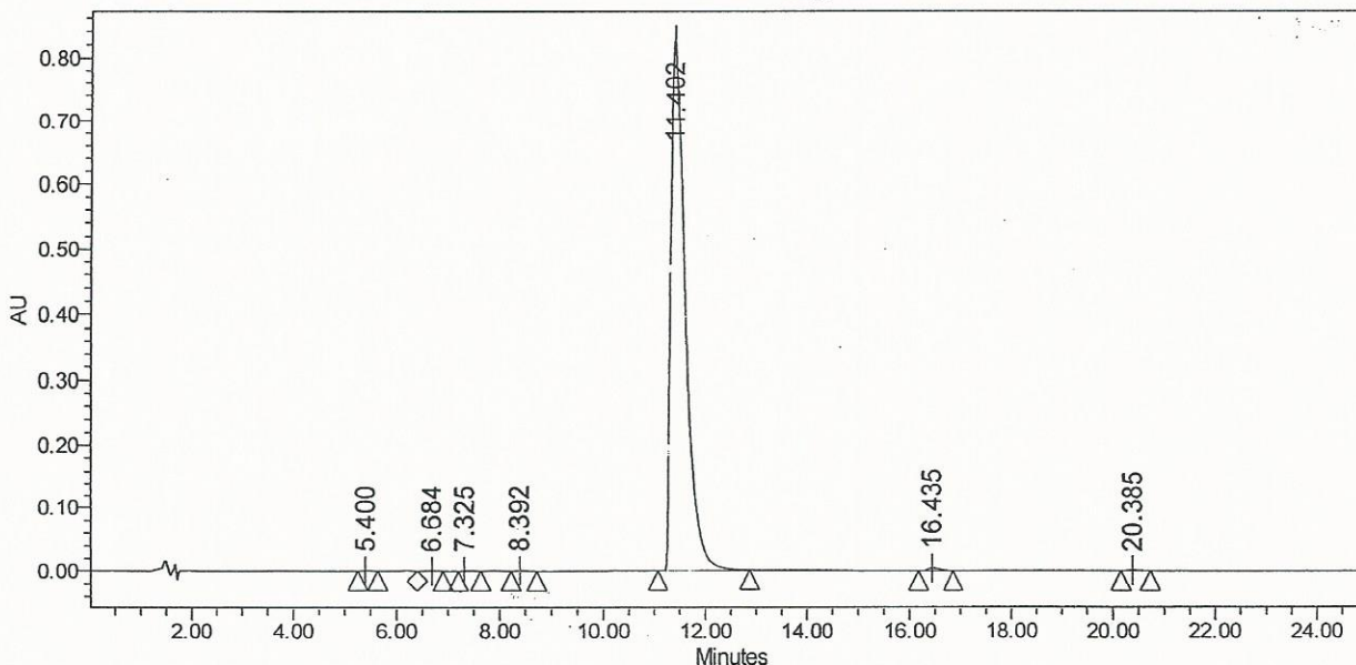
Auto-Scaled Chromatogram
